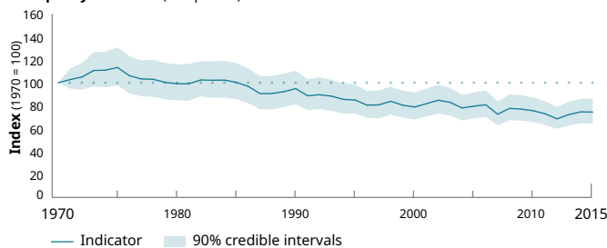
Occupancy indicator (14 species)
