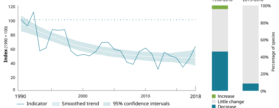
Abundance indicator (24 species)
