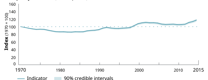
Occupancy indicator (1,265 species)
