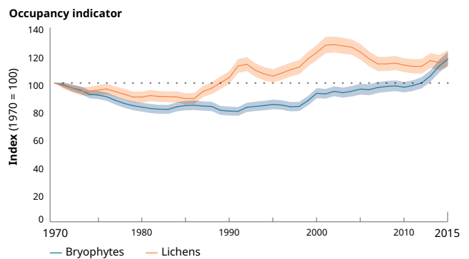
Change in the distribution for bryophytes (569 species) and lichens (696 species) 1970 to 2015
