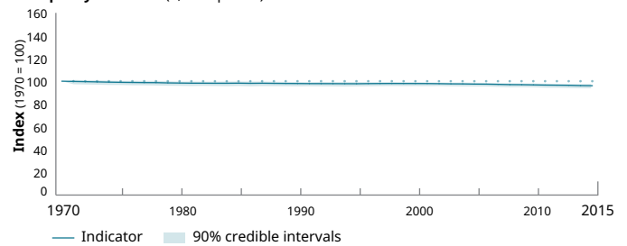
Occupancy indicator (1,351 species)
