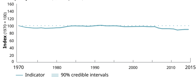
Occupancy indicator (3,162 species)
