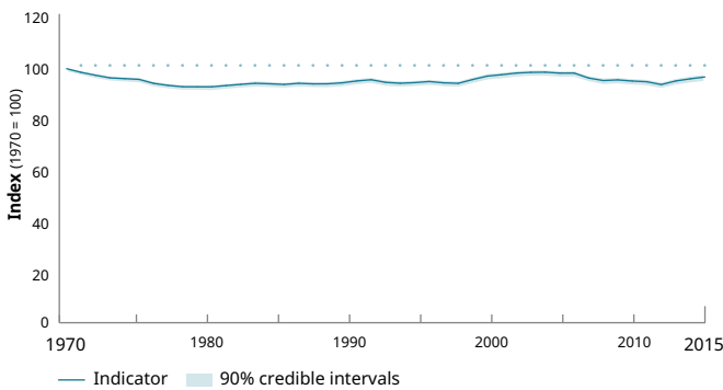
Occupancy indicator (6,654 species)
